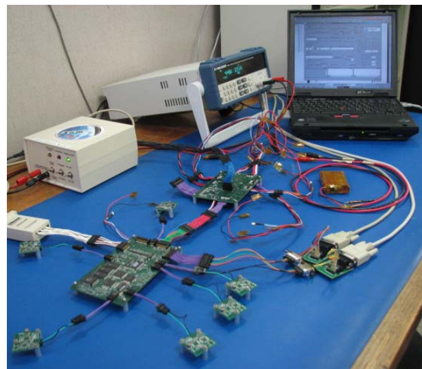
Figure 3. NTS Flatsat
